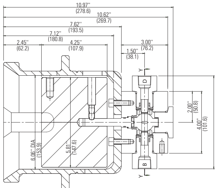
VIEW Z-Z
