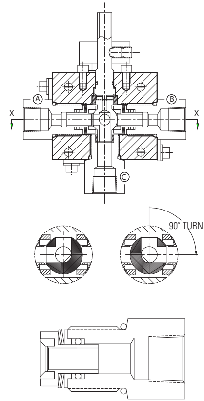
TYPICAL SIDE CONN
